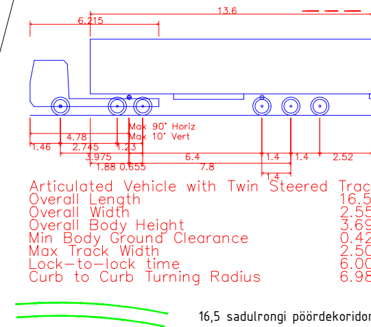
Articulated Vehicle with Twin Steered
